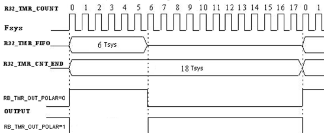
Figure 8-1 PWM output timing diagram
